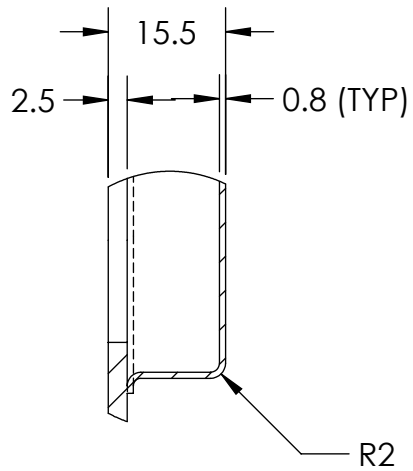
DETAIL B
