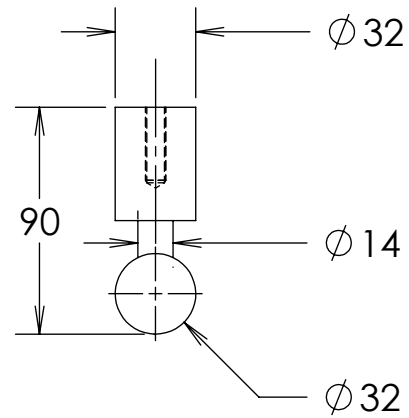
6400-32 SIDE VIEW
