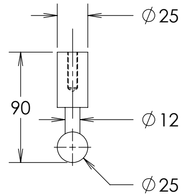
6400-25 SIDE VIEW
