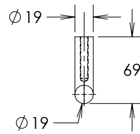
6200-19 SIDE VIEW
