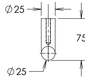
6200-25 SIDE VIEW
