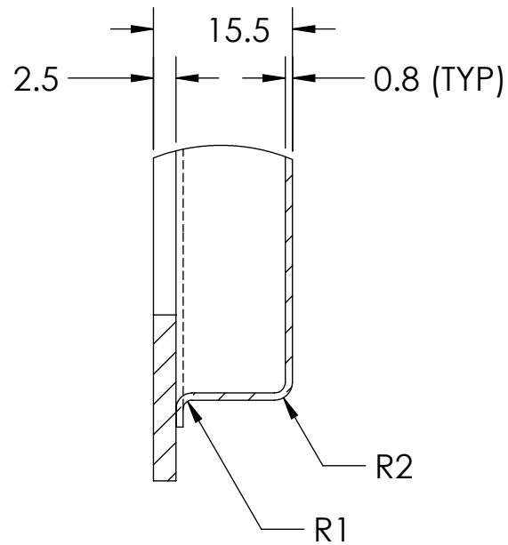
DETAIL B
